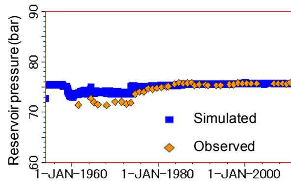
Fig. 13 The result of calculation of reservoir pressure (Reservoir G5).
